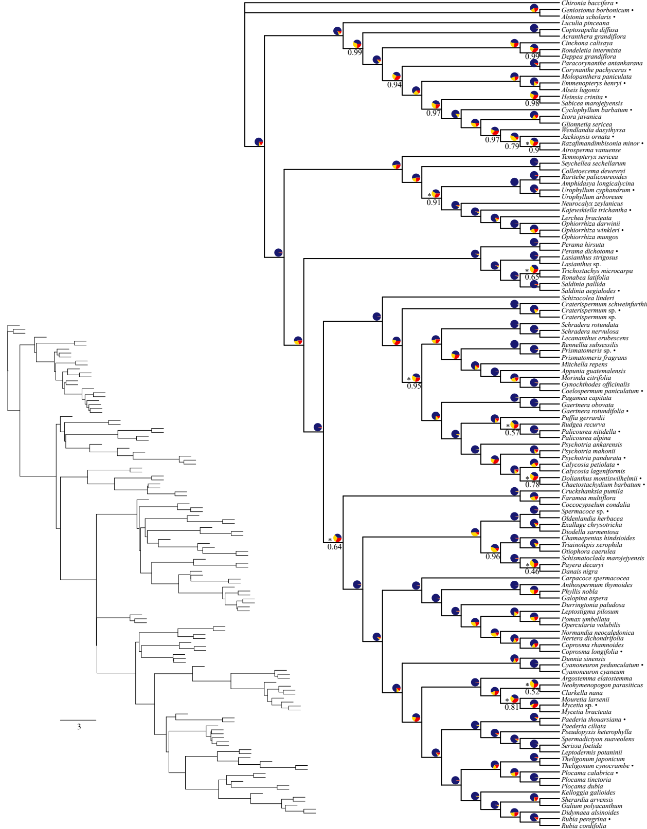
Supplementary Figure 3. Coalescent-based species tree estimated using ASTRAL on the paralog-filtered supercontig dataset. Numbers below branches denote local posterior probability (LPP) support values. Only support values smaller than 100% are shown. Pie charts show relative frequencies of the three quartet topologies around the branch (blue = congruent with species tree, yellow = first alternative topology, red = second alternative topology). Asterisks next to pie charts indicate failure to reject the hypothesis that the branch is a polytomy. Bullets after species names indicate samples downloaded from ENA. Inset shows branch lengths in coalescent units.
