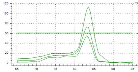
Figure S1. The melting curve of CNV1.
