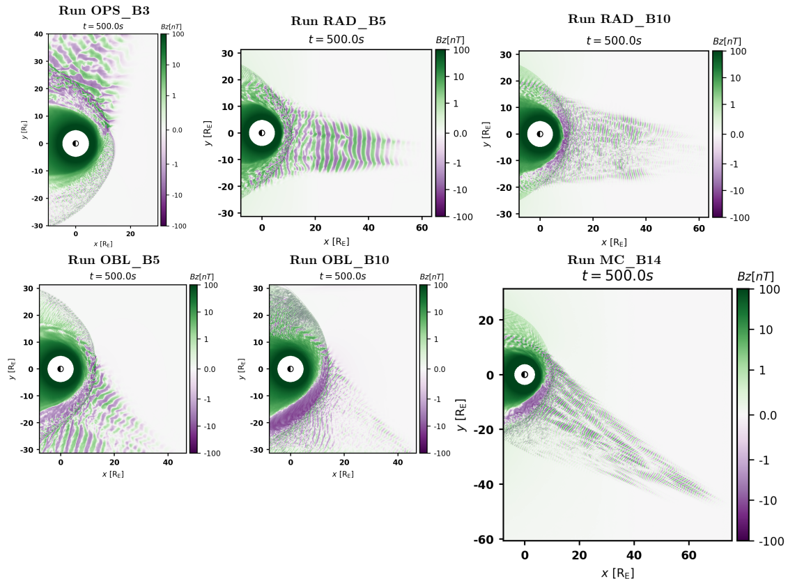
Figure S1. B_z magnetic field component in the runs under study at t = 500 s from the beginning of the simulation, in the entire simulation domain. This figure is similar to Figure 1 in the paper, but we show here the full extent of the simulation domain in each run.
