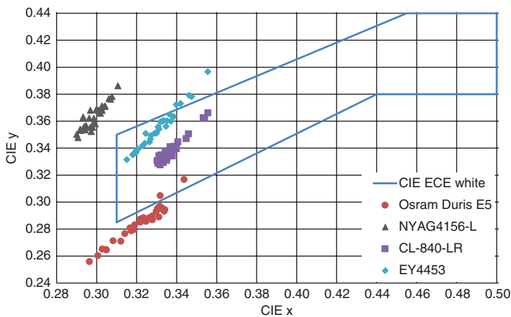
Figure 6 Chromaticity coordinates of selected phosphors at varied diode states [19].
