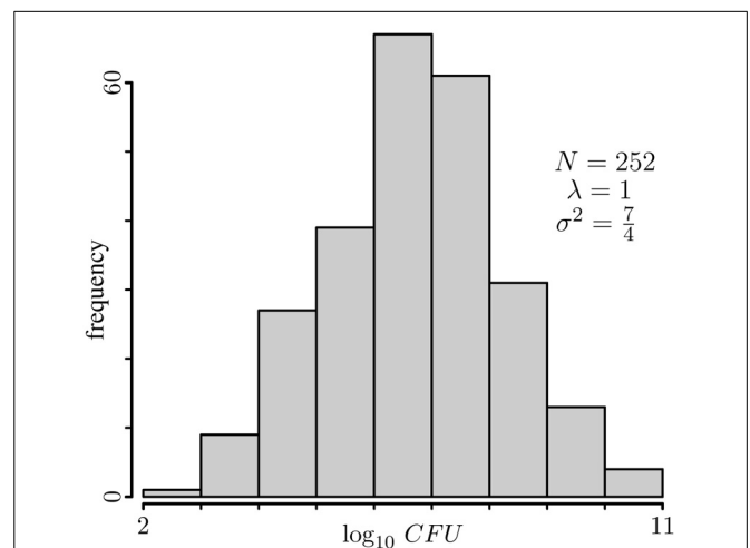
FIGURE 1 | Typical histogram of simulated data. The p -value profiles of the data on this histogram were computed and plotted in Figure 2 .
