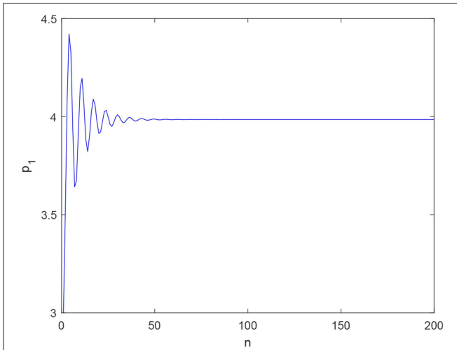
FIGURE 1 | Evolution of p_1 with \alpha = 0.2 .
