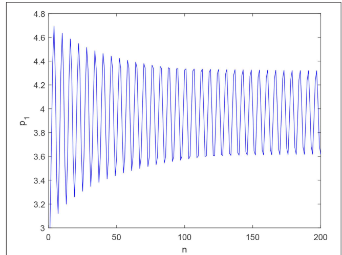
FIGURE 3 | Evolution of p_1 with \alpha = 0.176 .
