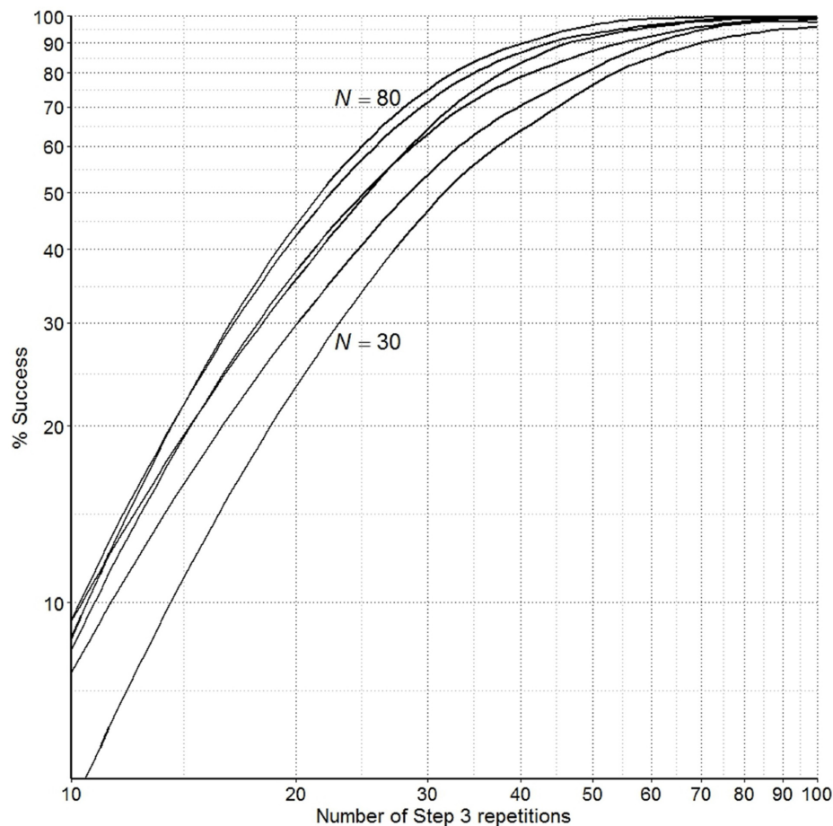
FIGURE 1 | Number of times out of 100 (% Success) the simulated random environmental walk precisely reproduced the rank order of the simulated 'participant's' preferences for 4 different simulated 'lighting applications' for group sizes N = 30 to N = 80 in increments of 10, for a given number of Step 3 repetitions from 10 to 100 in increments of 2.
