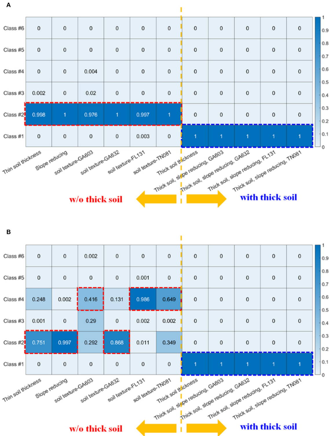
FIGURE 7 | The likelihood function L(y|F) as calculated by GMM in different PAWS+CLM experiments. Deeper blue color highlights higher probability. Here, we only show the (A) OR and (B) PIN subbasins, but the other 2 subbasins have similar results ( Appendix B ).
