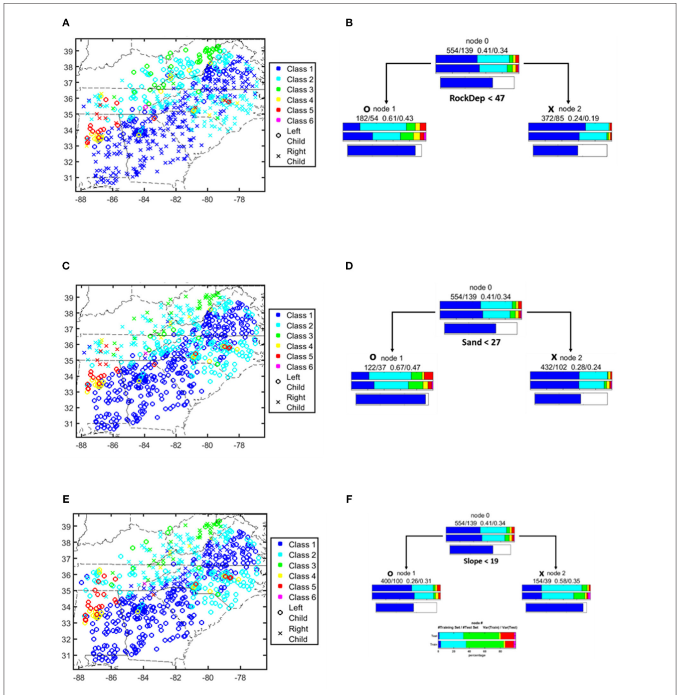
FIGURE 4 | A one-level classification tree model picks up soil thickness (RockDep) as the main difference between two types of storage-stream flow correlation patterns compared to other physical factors like soil texture (result for sand percentage shown here, Sand) and terrain (Slope) (Reproduced from FS17 with permission). (A,C,E) Southeastern region of CONUS. Color indicates SSCS class, symbols indicate tree nodes for physical factor (RockDep, Sand, Slope). (B,D,F) One-level ad hoc trees to predict class #1 in (A,C,E) via physical factor (RockDep, Sand, Slope).
