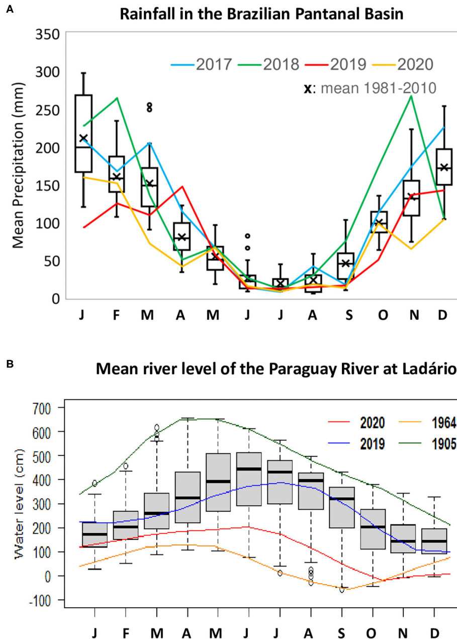
FIGURE 2 | (A) Annual variation of rainfall in the Brazilian Pantanal. Mean is indicated by “x” with the whiskers showing the standard deviation. Long-term mean is from 1981 to 210. The figure also shows rainfall for 2017, 2018, 2019, and 2020. Data is from CHIRPS. (B) Annual variation of levels of the Paraguay River at the Ladário gauge station. The figure also shows river levels for 1905, 1964, 2019, and 2020. Source of data: Brazilian Navy.
