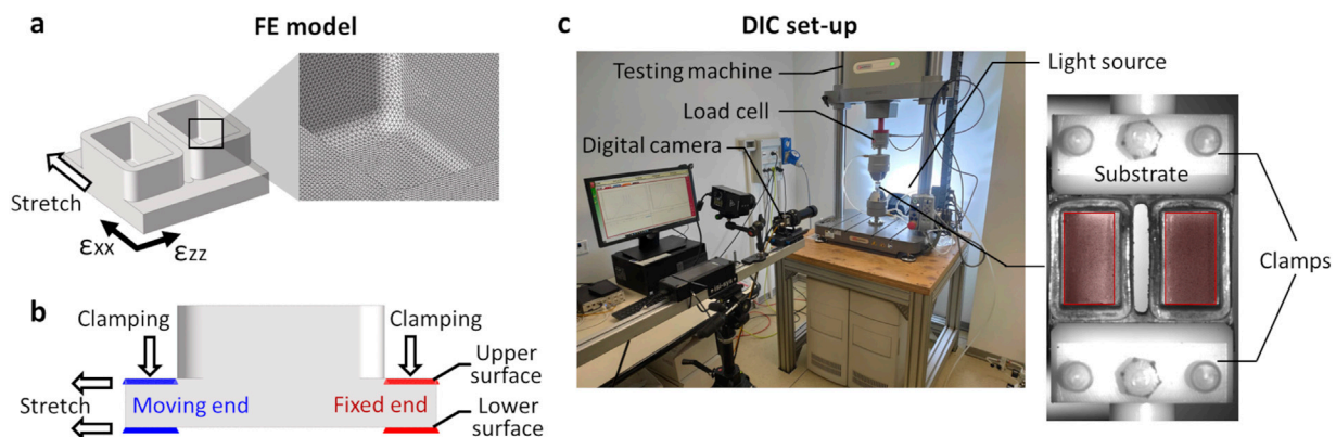
FIGURE 2 Mechanical characterization of S3 samples by computational and experimental methods. (a) Schematic drawing of the S3 sample geometry with strain reference directions and mesh (detail box). (b) Schematic drawing of the lateral view of the S3 sample, showing the boundary conditions applied during the clamping phase and the stretching phase with constrained (red) and moving (blue) nodes. (c) Experimental setup for mechanical characterization of the S3 samples. On the left, universal testing machine and digital image correlation (DIC) system. On the right, picture of the S3 sample acquired for DIC analysis showing the applied speckle. Red areas indicate the regions of interest (ROI) considered for strain computation.
