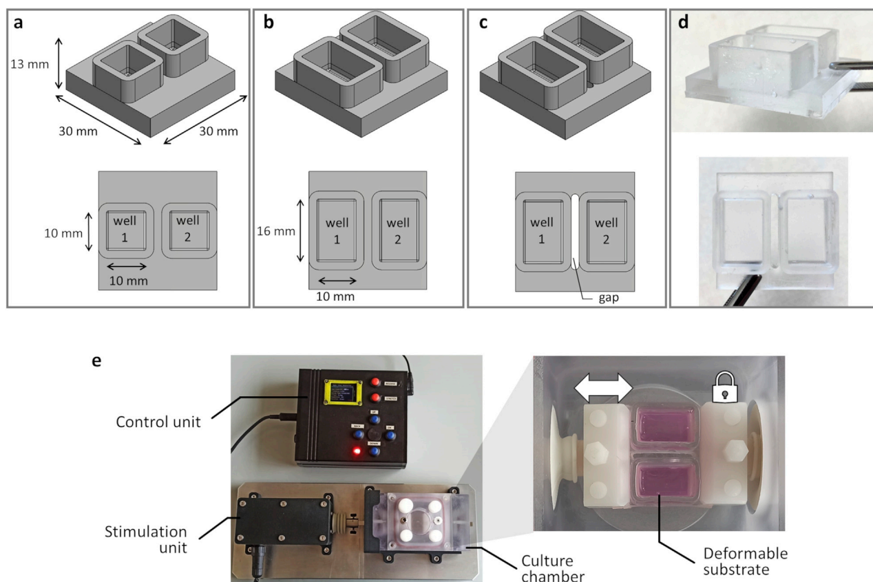
FIGURE 1 Deformable substrate versions and investigation platform. 3D models of the substrate versions and top view (on bottom) showing the substrate geometrical features and dimensions: (a) S1 version; (b) S2 version; (c) S3 version. (d) S3 version manufactured in PDMS. (e) Investigation platform composed of the automated stretch bioreactor, with the control unit, the stimulation unit, and the culture chamber, housing the S3 mounted in the clamping system.
