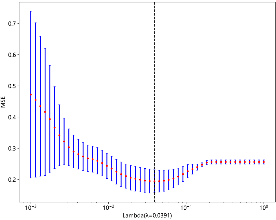
FIGURE 4 The MSE of LASSO regression.
