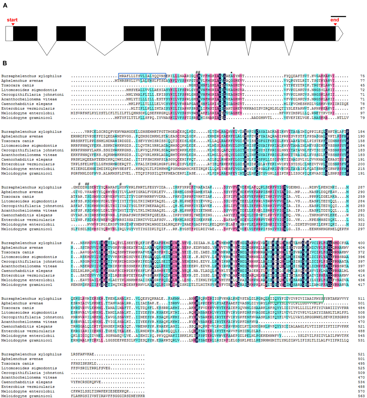
FIGURE 1 | Sequence analysis of UGT440A1 . (A) Genomic DNA structure of UGT440A1 . White boxes indicate exons, the black region corresponds to the coding sequences, and the lines indicate introns; scale bar = 100 bp. (B) Alignment of UGT440A1 with homologs. The alignment compares UGT440A1 (M2467299) with the UGT proteins of Aphelenchus avenae (KAH7725749.1), Toxocara canis (KHN83392.1), Litomosoides sigmodontis (VDK69150.1), Cercopithifilaria johnstoni (CAG9530659), Acanthocheilonema viteae (VBB30777.1), Caenorhabditis elegans (NP_506211.1), Enterobius vermicularis (VDD95930.1), Meloidogyne enterolobii (CAD2191161.1), and Meloidogyne graminicola (KAF7639096.1). Black, red, and blue shades indicate fully conserved, strongly conserved, and weakly conserved amino acids, respectively. Signal peptide sequences, transmembrane region, and typical signature of UGT are enclosed by the blue, green, and red boxes, respectively. The predicted active sites and polypeptide binding sites are indicated by (#) and (*), respectively.
