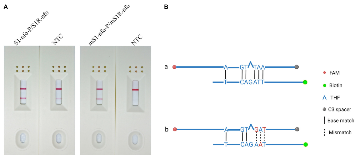
FIGURE 3 | Preliminary test and analysis of the original primer-probe set and base-substituted primer-probe set. (A) The image shows the LFD results for RPA amplifications using original primer-probe set and base-substituted primer-probe set. The name of each set is displayed above dipstick. NTC is no template control tested for false-positive signals. The positions of test and control lines are marked on the right of the dipsticks image. The template was B. xylophilus gDNA. The reactions are carried out at 38°C for 10 min. (B) Analysis of the cross-dimer formation between the probe and reverse primer. The original probe has five-continuous base pairings with original reverse primer, which could lead to primer-probe complex, resulting in a false positive signal. After bringing in mispairings into the original self-ligating primer-probe set, one of which is on reverse primer and two on the probe, the formation of the probe-primer complex is artificially interrupted and signal is eliminated. Labels and modifications for DNA, nfo, base matches, and mismatches are represented by different shapes and colors, and a legend is given to the right of the figure. Created with BioRender.com.
