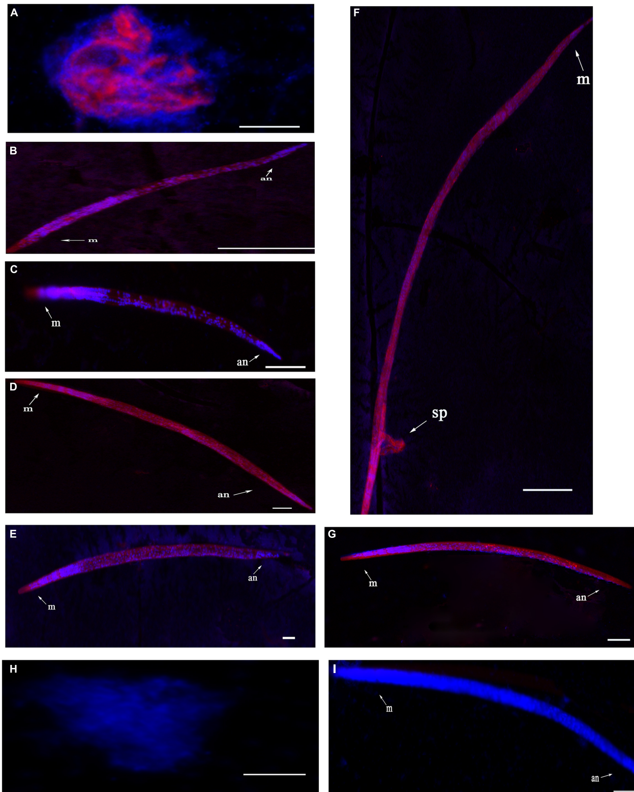
FIGURE 4 | Localization of UGT440A1 mRNA in B. xylophilus determined through fluorescence in situ hybridization. Hybridization with the red fluorescence-labeled probes in the embryo (A), J2 juvenile (B), J3 juvenile (C), male J4 juvenile (D), female J4 juvenile (E), male adult (F), and female adult (G). Hybridization in embryo (H) and female adult (I) in the negative control. m, metacarpus; an, anus; sp, spicules. Scale bar = 20 \mu m (A–E, H), 50 \mu m (F, G, I).
