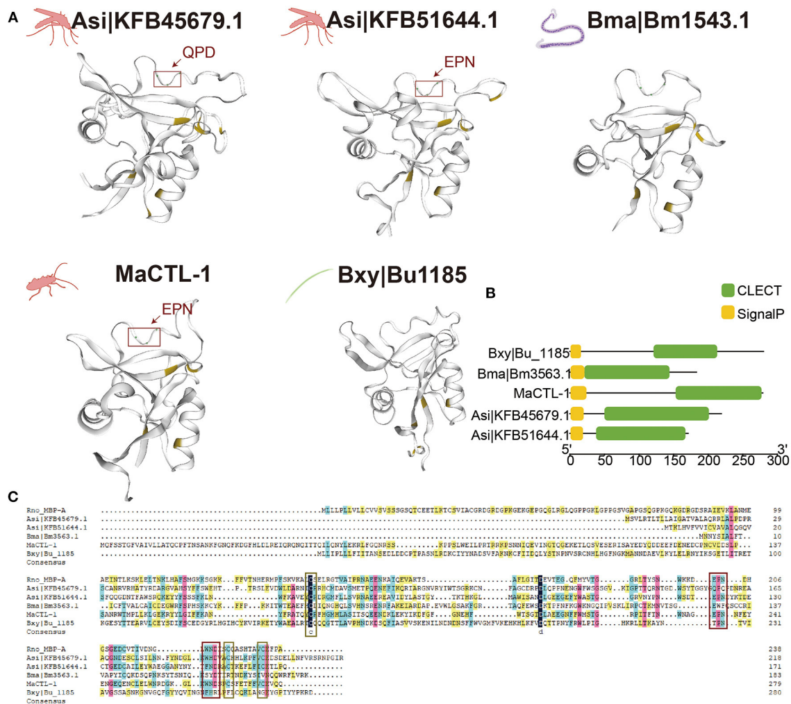
FIGURE 4 | Similarity of nematode and their insect-vector lectins. (A) Structural model of the carbohydrate-recognition domain (CRD) of Bxy|Bu_1185, MaCTL-1, Bma|Bm1543.1, Asi|KFB45679.1, and Asi|KFB51644.1. Cysteine is shaded in yellow, and carbohydrate-binding motif is underlined in the red box. (B) Schematic structure of CTLs. The putative signal peptide (SP), CTL, are indicated in different color boxes. (C) Alignment of the amino acid sequences of Bxy|Bu_1185 in B. xylophilus , Bma|Bm1543.1 in B. malayi , MaCTL-1 in M. alternatus , and Asi|KFB45679.1 and Asi|KFB51644.1 in A. sinensis . Domain abundant in cysteine is underlined in the yellow box and carbohydrate-binding motifs are underlined in the red box.
