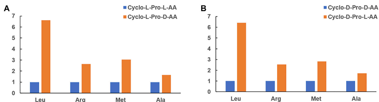
FIGURE 4 | The relative intensity of UV-absorption of the cyclo-Pro-AA at 210 nm in these reactions. (A) Bar graph representation of the reaction L-Pro with four L-/D-AAs, respectively. (B) Bar graph representation of the reaction D-Pro with four L-/D-AAs, respectively.
