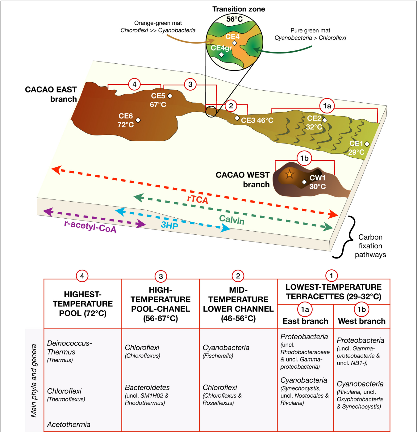
FIGURE 5 | Ecological reconstruction of the microbial community distribution along the Cacao hydrothermal transect based on lipid biomarkers and DNA sequencing. The hydrothermal ecosystem was defined by a succession of microbial community structures and metabolic traits along the temperature gradient, with dominance of thermophilic species at high temperature, of anoxygenic photosynthetic species at intermediate temperatures (67–46°C), and mesophilic and oxygenic photosynthetic species at low temperature (≤32°C). In the channel, the compositional and metabolic transition at 56°C represented an ecological tipping point where aerobic and anaerobic conditions may alternate (from coexistence of Cyanobacteria and Chloroflexi to dominance of Chloroflexi and from a Chloroflexi community, largely photoheterotrophic to one mostly photoautotrophic). The abbreviation “uncl” means unclassified.
