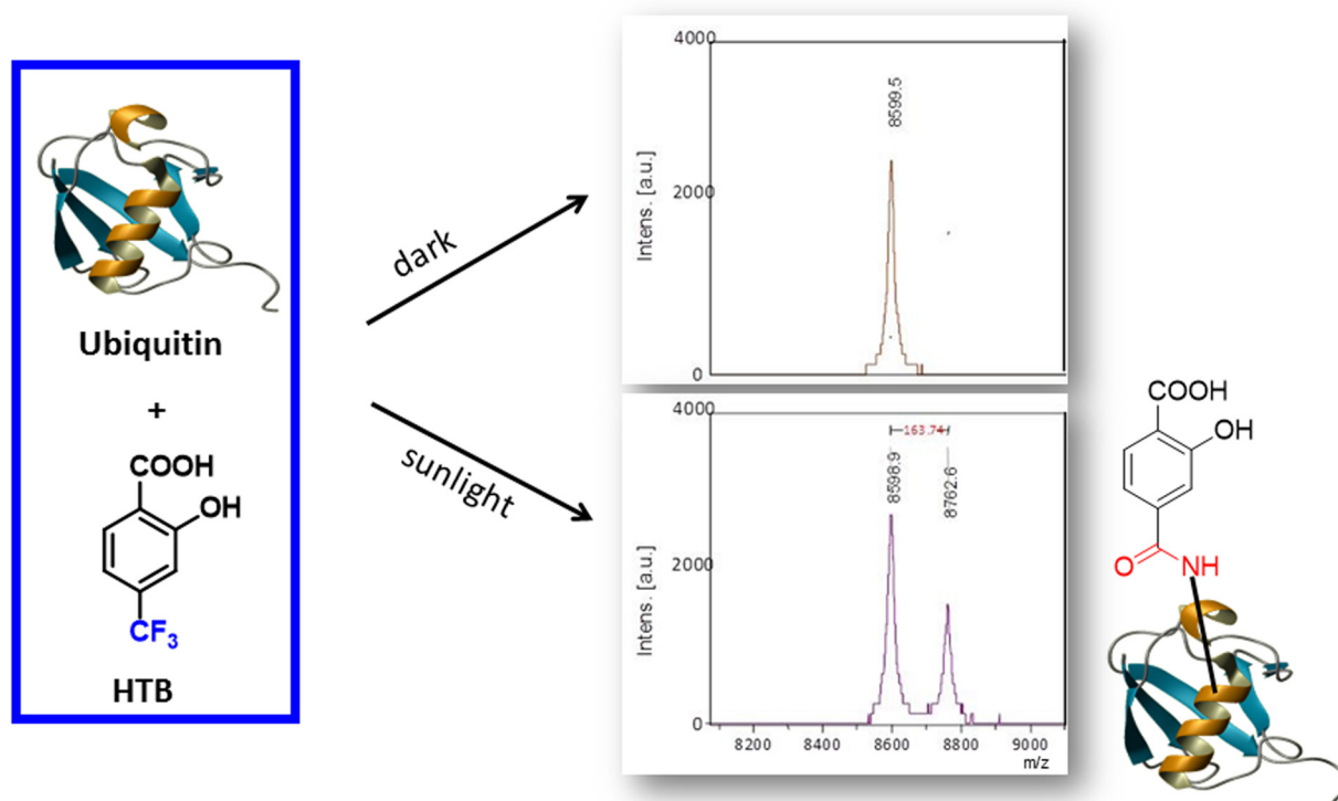
FIGURE 6 | MALDI-TOF spectra of HTB-ubiquitin (10:1) kept in the dark (Top) or solution after 30 min of sunlight irradiation (Bottom).
