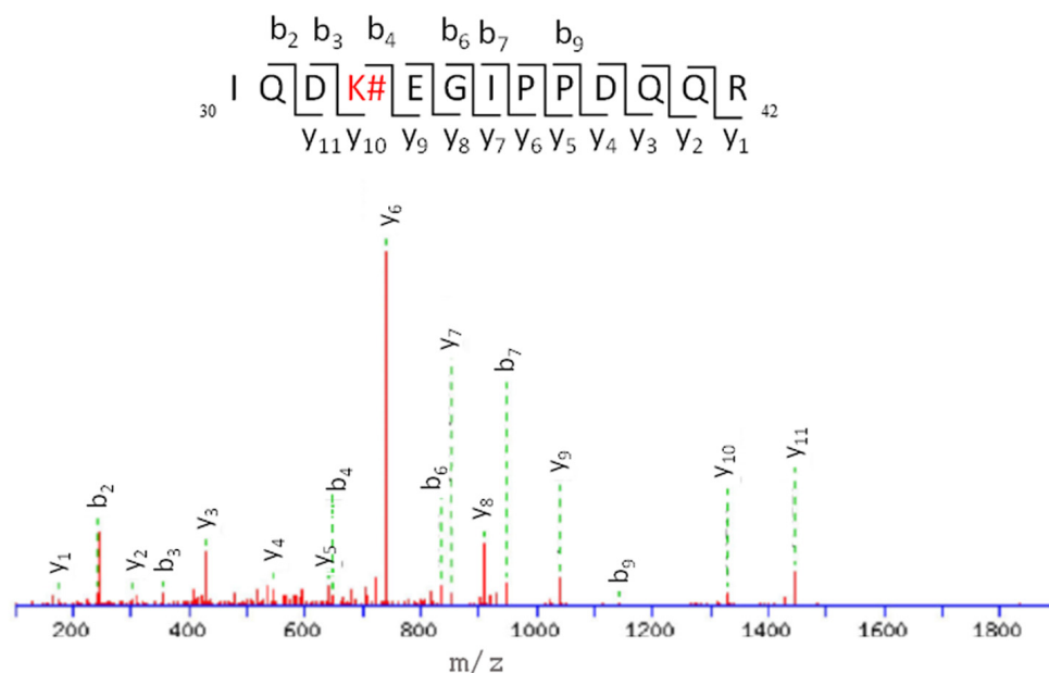
FIGURE 7 | ESI-MS/MS spectra and fragmentation pathway of the HTB-modified peptide 4.
