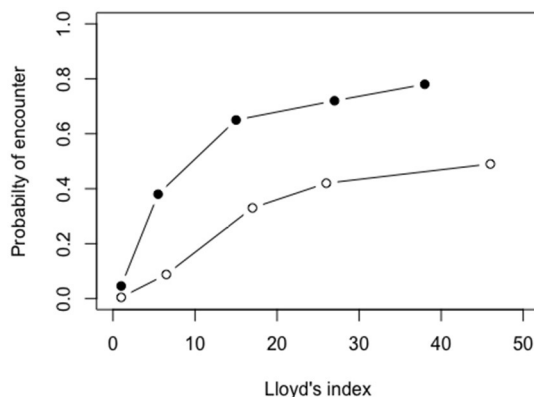
FIGURE 4 | Encounter probabilities of passive larvae as a function of the patchiness of initial larval distribution, implementing high ( 0.026 \text{ ind m}^{-3} ; full circles) and low ( 0.0026 \text{ ind m}^{-3} ; empty circles) larval densities. Simulations were carried out in the 3D biophysical model within a sub-sample of 100 \times 100 \times 100 \text{ m} (length \times width \times depth) in the Gulf of Aqaba centered around 29^\circ 29.4' \text{ N } 34^\circ 57.4' \text{ E} during the 15th of March 2004 at 12:00–12:10 p.m.
