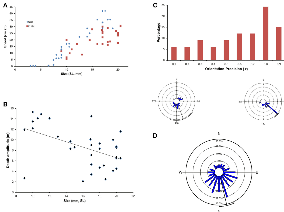
FIGURE 1 | (A) Ontogenetic change in swimming speed as measured in a laboratory raceway (critical speed [Ucrit], Diamonds), and in the ocean ( in situ speed, Squares) of a serranid, Epinephelus coioides . Note the wide range in speeds at any size, particularly in the ocean. Although there is a significant increase in speed with size for both measures, the laboratory measure relationship explains 92% of the variation over the common size range whereas the in situ relationship explains only 54%. Data from Leis et al. (2007, 2009). (B) Ontogenetic change in in situ depth amplitude (difference between greatest and least depth) in larvae of a serranid, Epinephelus coioides . Note the wide range in depth amplitude at any size. The significant ontogenetic decrease in depth amplitude explains only 25% of the variation. Size of larvae is standard length (SL). Data from Leis et al. (2009). (C) Frequency distribution of in situ orientation precision ( r , length of the mean vector) of 33 individual larvae of a serranid, Epinephelus coioides . The circular insets show the distribution of swimming bearings of two individuals measured every 30 s over a 10 min observation period. Although both individuals have significantly directional swimming to the South-East, the one on the left ( r = 0.43 , p = 0.02 ) has a more meandering swim path than the one on the right ( r = 0.89 , p < 0.0001 ). Data from Leis et al. (2009). The thin black radius is the mean direction, and the arc at its end is the 95% confidence interval. (D) In situ directional swimming by larvae of a pomacentrid, Chromis tripteron , off the west side of Lizard Island, Great Barrier Reef, showing the frequency distribution of mean swimming bearings of 205 individually measured larvae with significant within-individual swimming directionality. The among-individual swimming direction was to the South-South-East (mean = 166.7 ± 12.8°), and highly significant ( p < 0.0001 , Rayleigh Test), but 22% of larvae swam in a direction that differed more than 90° from the mean. Data from Leis et al. (2014).
