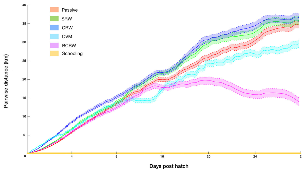
FIGURE 3 | Distances between pairs of virtual larvae that hatched at the same locations and times throughout the pelagic larval duration (PLD) for the following strategies: passive, simple random walk (SRW), auto-correlated directional swimming (CRW), ontogenetic vertical migration (OVM), biased correlated random walk (BCRW), and schooling behavior (simulation #3–8, Table 1 ). Shaded areas indicate 99% confidence intervals ( N = 32,046 and 28,414 for the passive and other strategies respectively).
