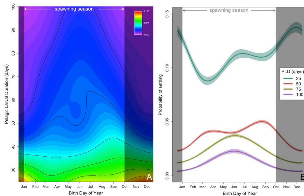
FIGURE 3 | (A) Predicted probability of settling (contours and color scale), from high (red) to low (purple) probability, as a function of birth date (x-axis, BirthDay ) and PLD (y-axis, days). (B) Predicted probability of settling ( \pm 2 standard error) as a function of birth date of year ( BirthDay ) and PLD (days, colors, with green = 25 days, red = 50 days, yellow = 75 days, and purple = 100 days). In both panels, times outside the common spawning season are shaded in gray (Walsh, 1987; see section Discussion). Other predictors are held constant at Location = Punalu'u, Spine = present, Moon = New.
