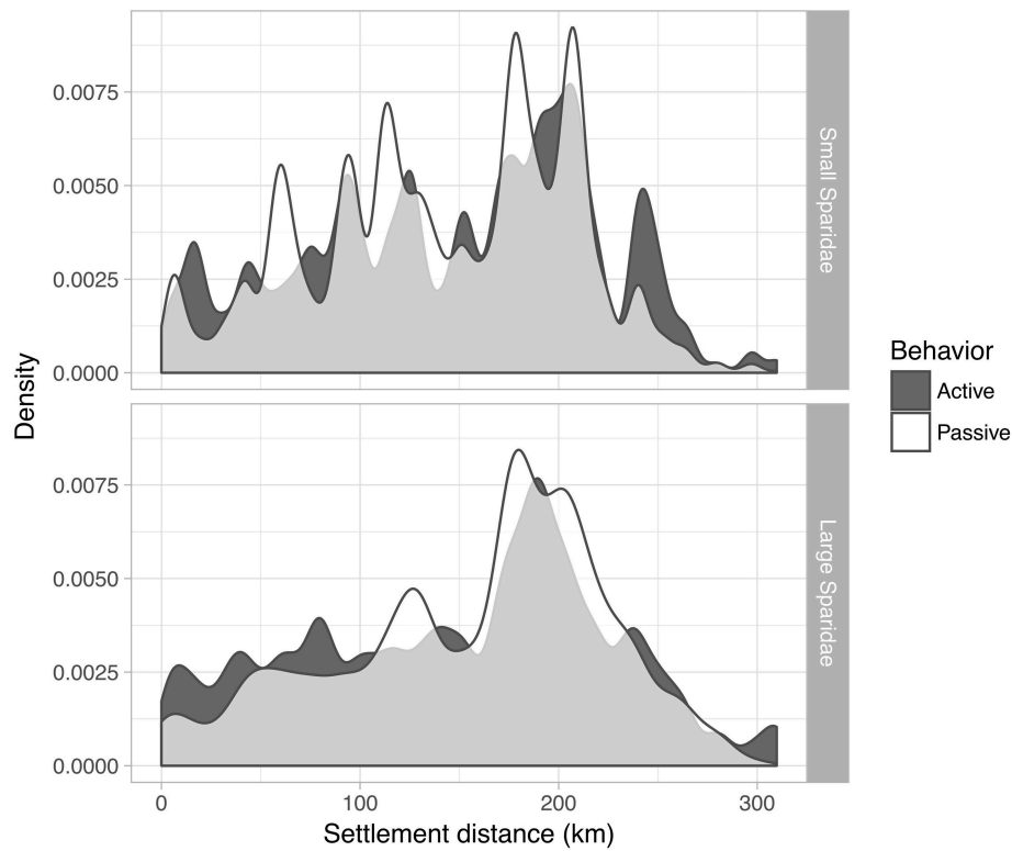
FIGURE 6 | Dispersal kernels for the two groups of Sparidae and the two simulation configurations, i.e., kernel density smoothing of distances from the release site to the settlement site.
