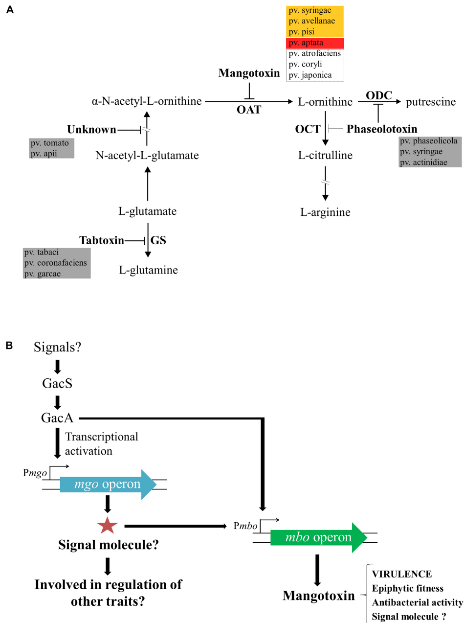
FIGURE 3 | Enzymatic target of mangotoxin and its biosynthesis regulation. (A) Representative scheme of the arginine-glutamine and polyamine biosynthesis pathways. The enzymatic targets of the different antimetabolite toxins, including mangotoxin, and the different pathovars involved in the production of the different antimetabolite toxins are depicted. OAT, ornithine N -acetyltransferase; OCT, ornithine carbamoyltransferase; ODC, ornithine decarboxylase, and GS, glutamine synthetase. Orange box: pathovars positives for the presence of mbo genes and positives for mangotoxin production; red box: pathovar positive for the presence of mbo genes, but negative for mangotoxin production; dotted lines box: pathovars positive for the presence of mbo genes, but not experimentally tested for mangotoxin production. (B) Mangotoxin biosynthesis regulation model. GacS/GacA two-component regulatory system regulates directly or indirectly the transcription of the mgo operon. Mgo operon could synthesize a positive regulator (signal molecule) to activate the mbo operon transcription. The mbo operon produces mangotoxin, which acts primarily as a virulence factor, although, other functions have been described.
